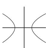
(c) Hyperbola
