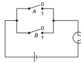
(a) Switching circuit for or-function
