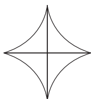
(f) Astroid
