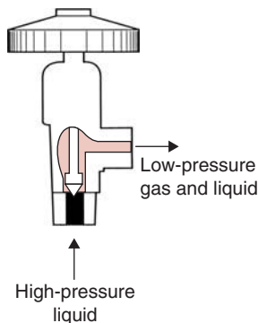
■ Figure 6.12 A manually operated expansion valve. (Courtesy of Carrier Co.)
