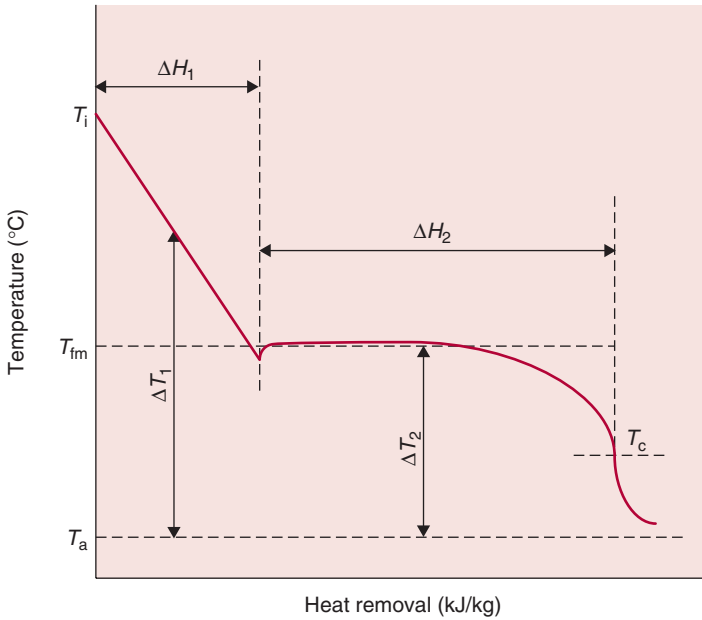
■ Figure 7.17 Freezing diagram of food, divided into sections for Pham's method.
