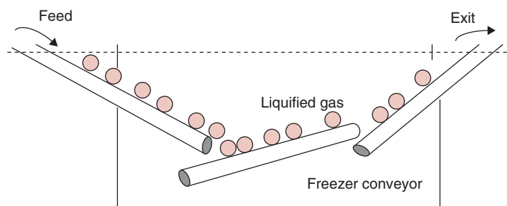
Figure 7.8 Schematic illustration of an immersion freezing system.
