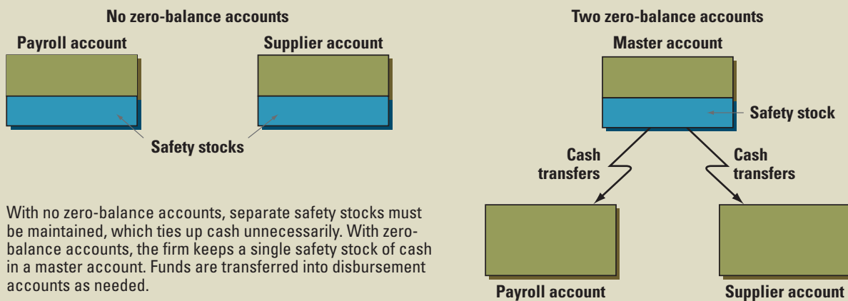
Figure 27.5 Zero-Balance Accounts
