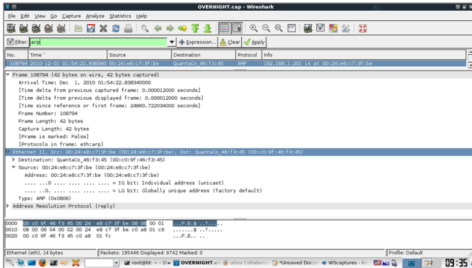
Figure 6-1: Layer 2 headers
